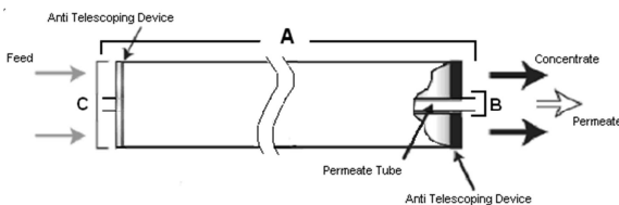
Figure 2: Element Dimensions Diagram – Male (4040)
